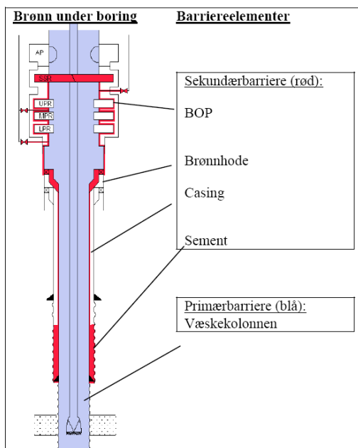
Figur 19 Barriereskjema vist for en brønn under boring (Ref. 44)
