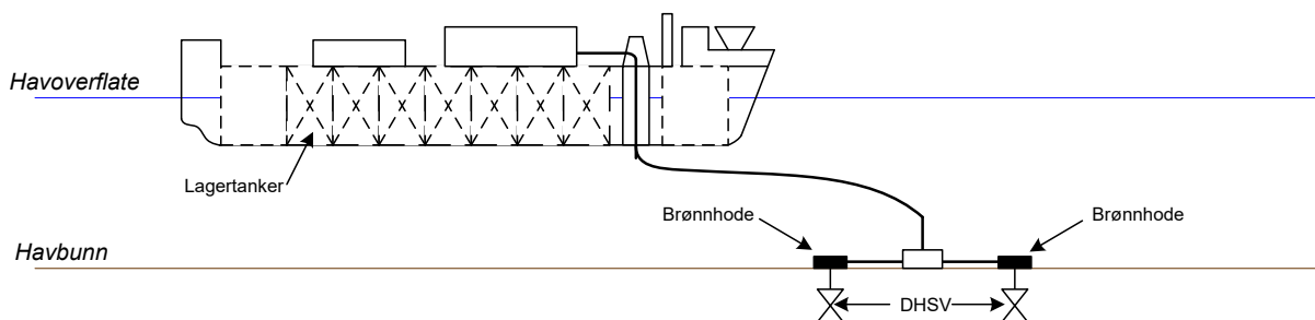
Figur 5 FPSO
