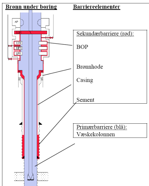
Figur 19 Barrierskjema vist for en brønn under boring (Ref. 44)
