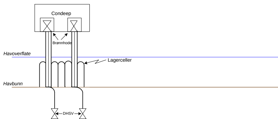
Figur 7 Condeep
