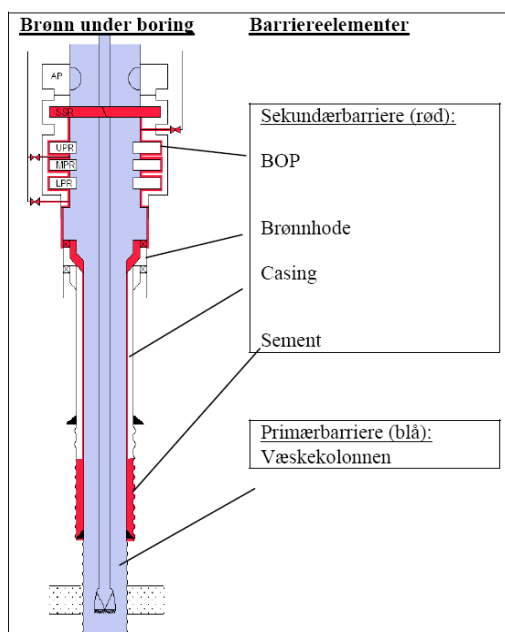
Figur 19 Barriereskjema vist for en brønn under boring (Ref. 45)
